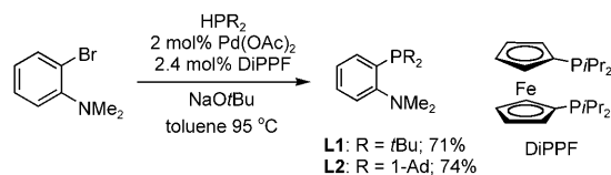
Scheme 1. Synthesis of ligands L1 and L2 by P–C cross-coupling.
