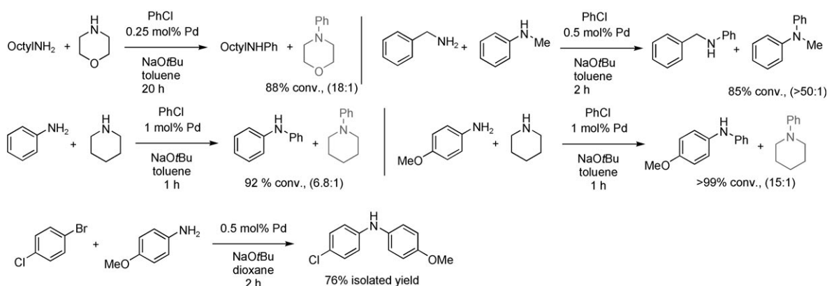
Scheme 2. Chemoselective C–N cross-coupling reactions. All reactions employ [\text{Pd}(\text{cinnamyl})\text{Cl}]_2 and L2 (Pd/L 1:2), with conversions and product ratios determined on the basis of GC data unless indicated.
