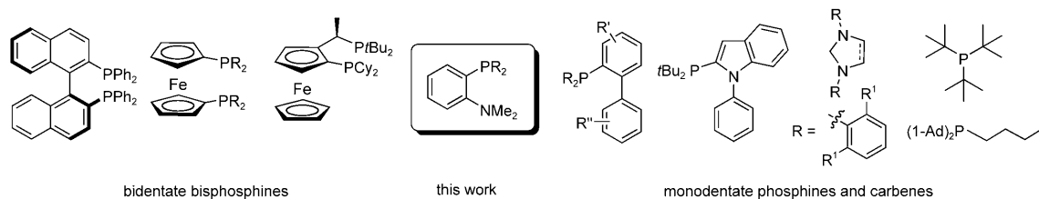
Figure 1. Selected examples within the evolution of ligands for Pd-catalyzed C–N cross-coupling reactions.
